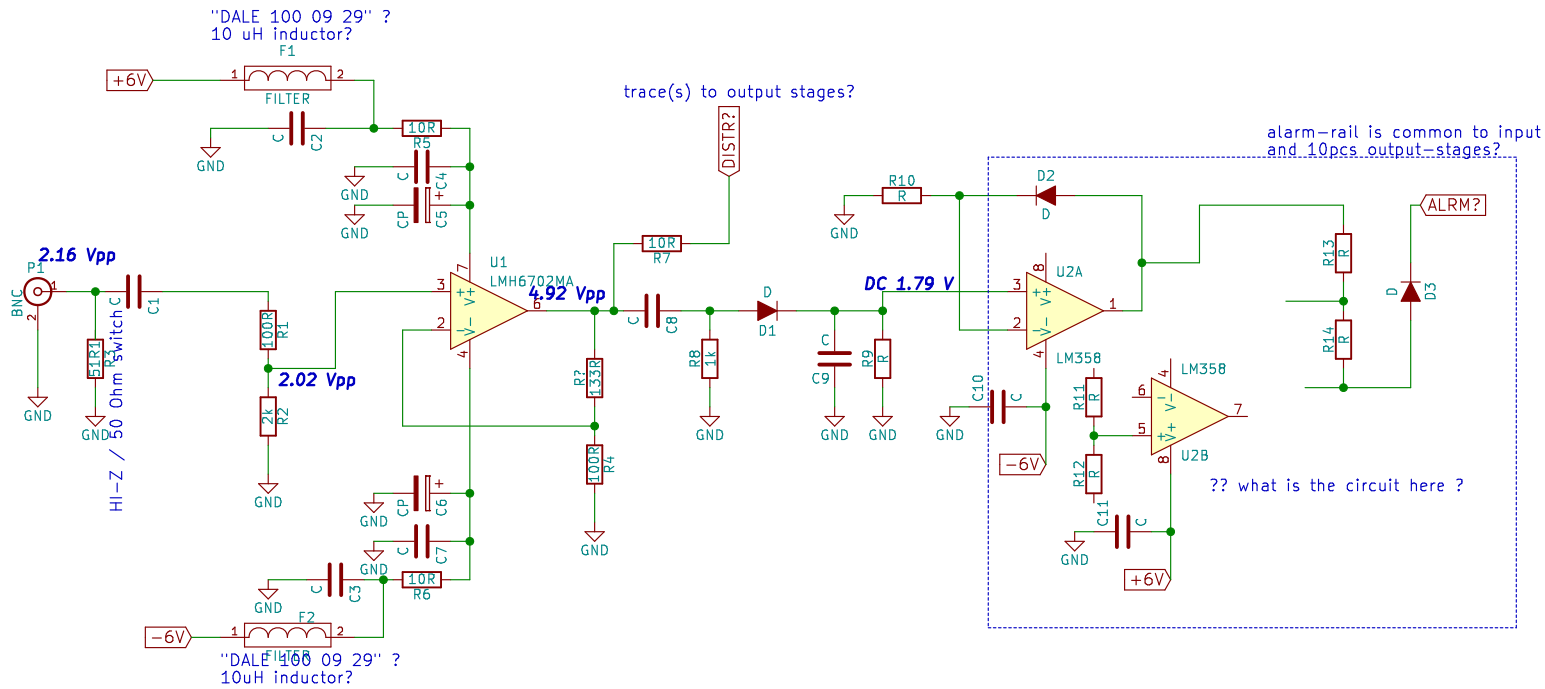
INPUT stage
